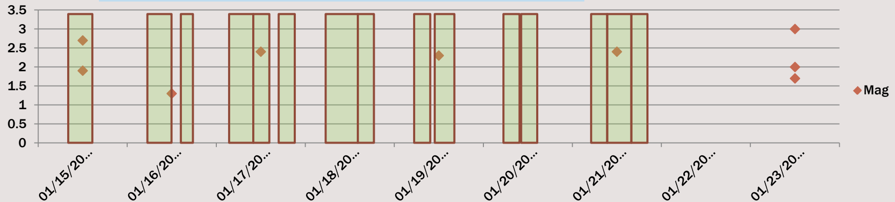
Overall facing window, 15 stages in 3 wellbores, Jan 15 to 21
